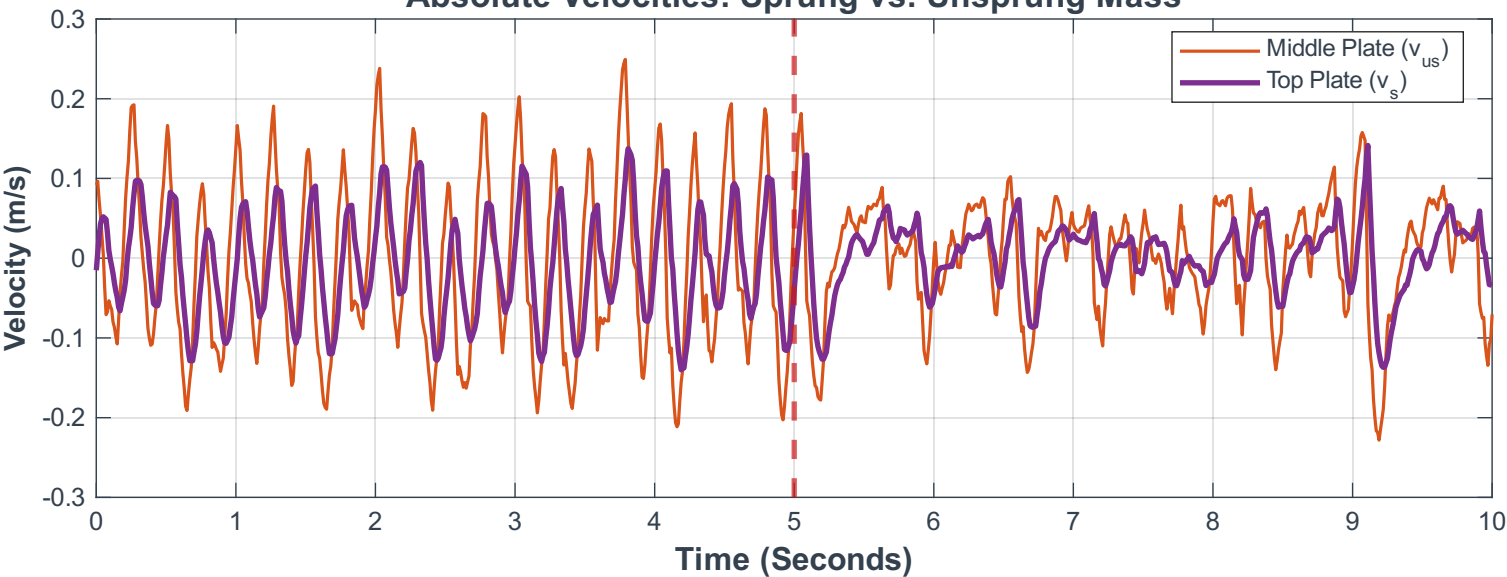
Absolute Velocities: Sprung vs. Unsprung Mass
