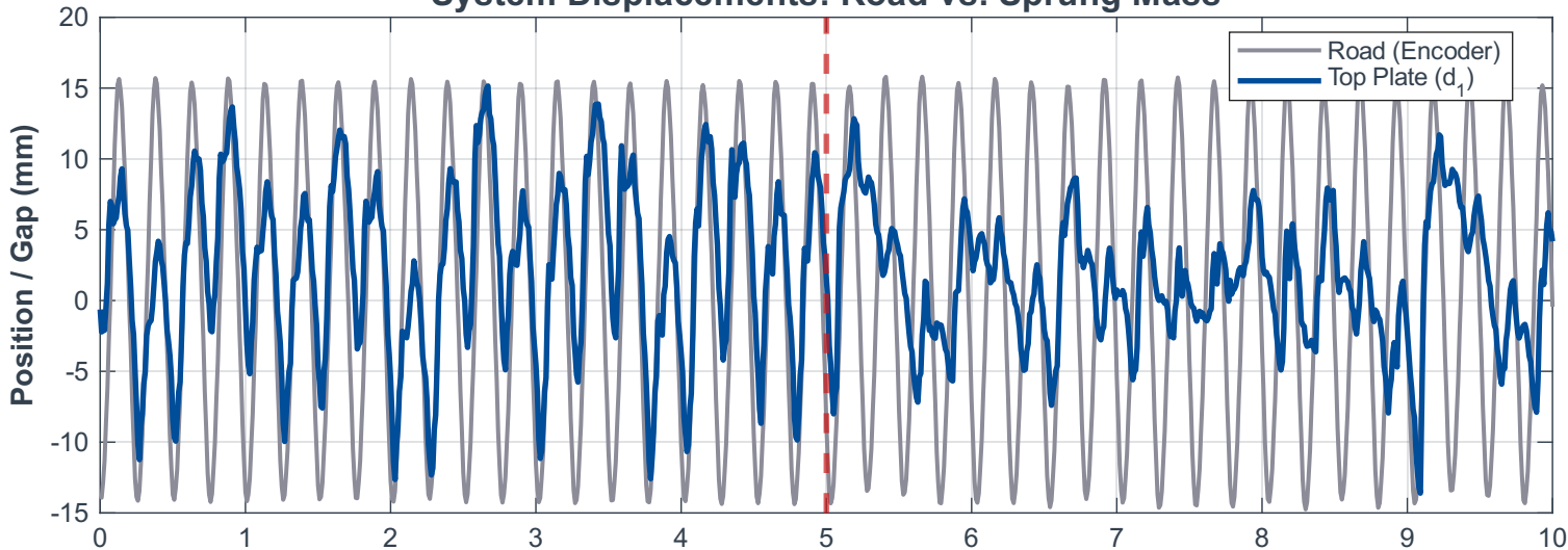
System Displacements: Road vs. Sprung Mass
